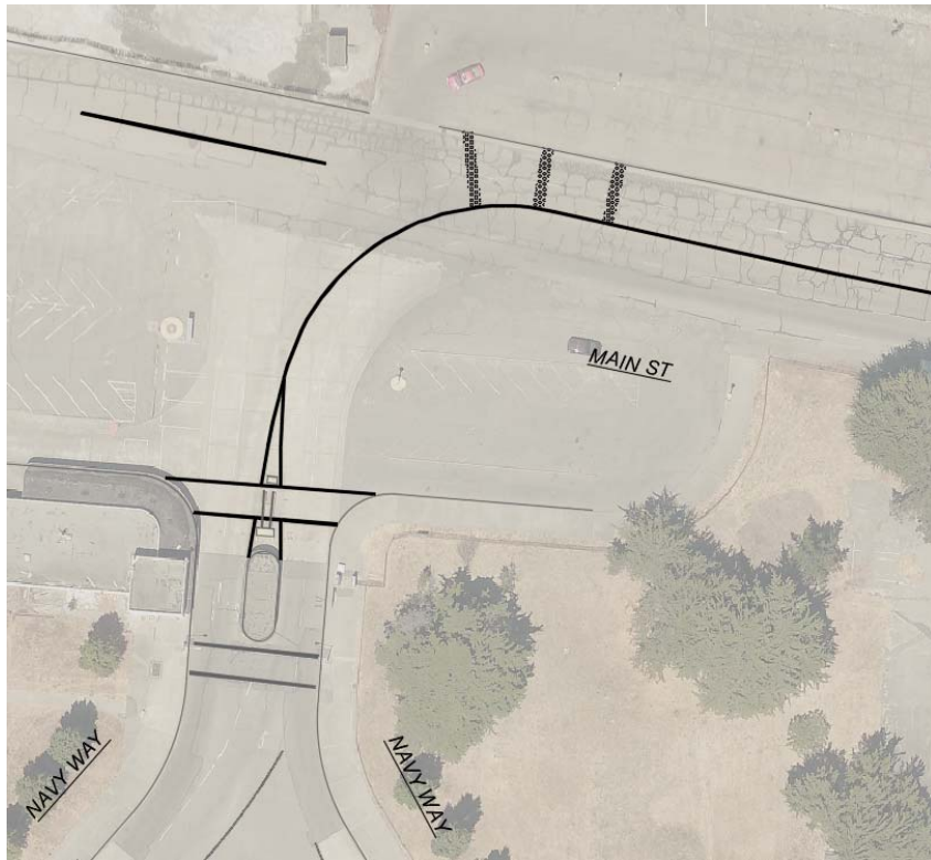
Main Street at Navy Way. Existing Conditions (top) and Proposed Improvements (bottom).
