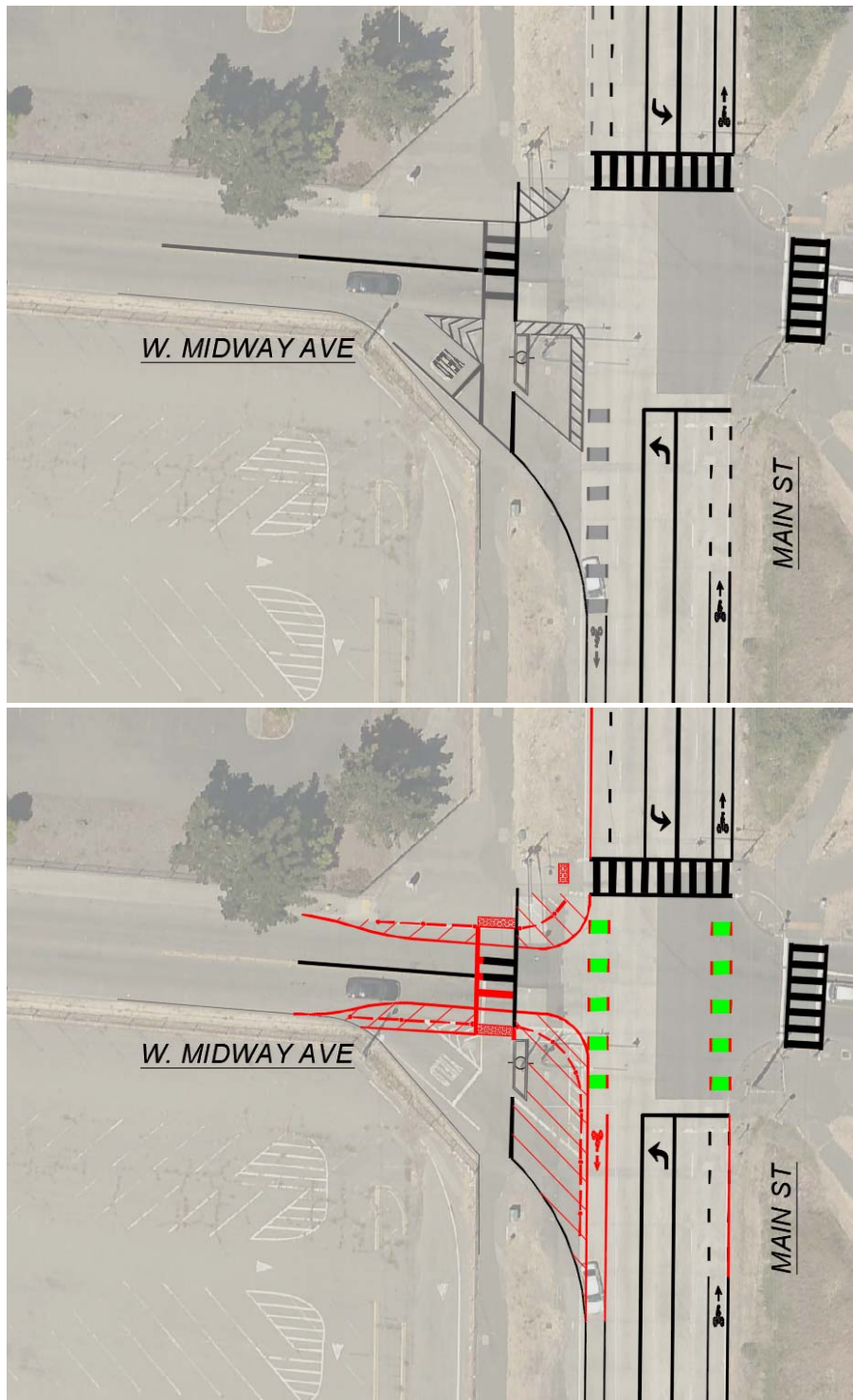
Main Street at W. Midway Avenue. Existing Conditions (top) and Proposed Improvements (bottom).
