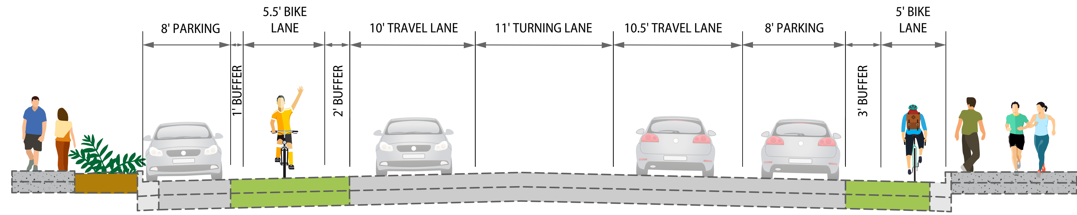
SECTION B-B
