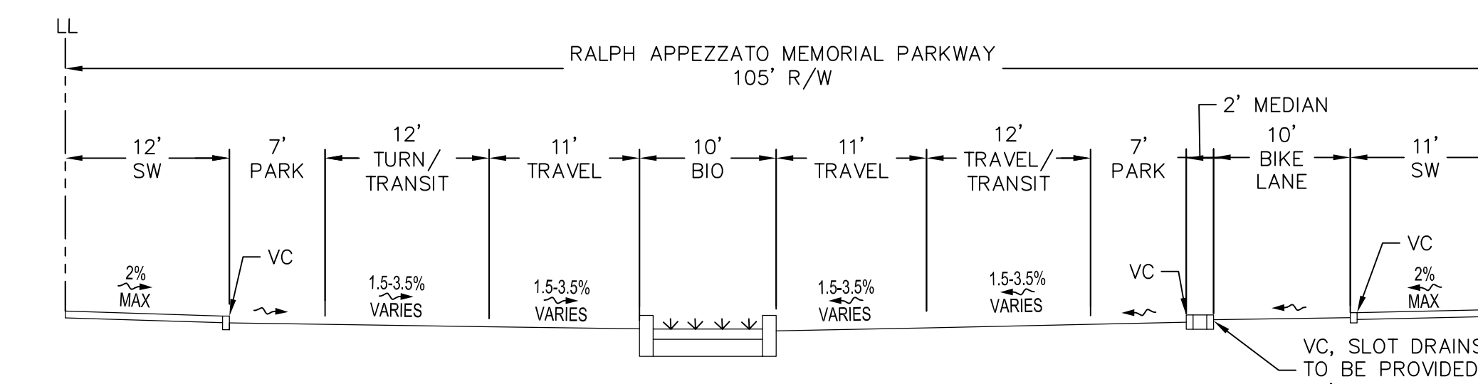
D RALPH APPEZZATO MEMORIAL PARKWAY NTS
