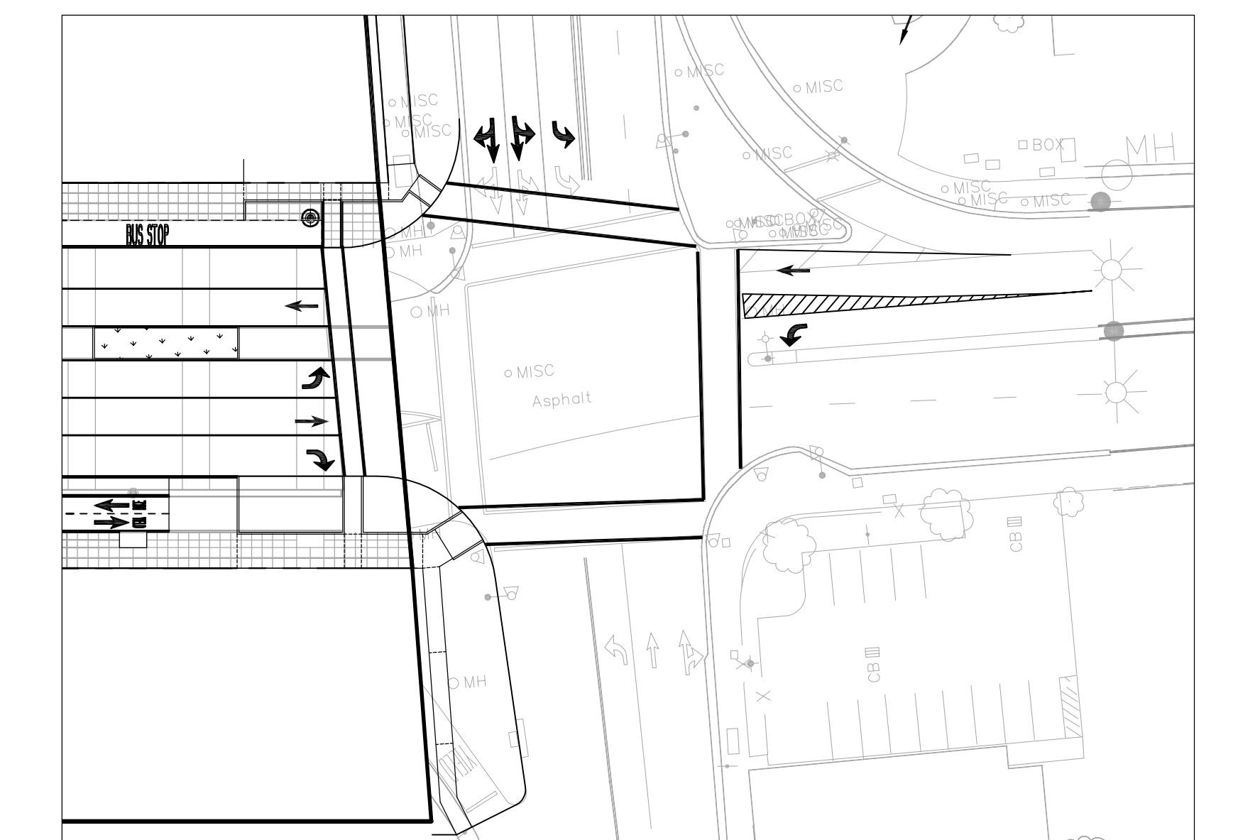
INTERIM MAIN STREET/RAMP INTERSECTION SCALE: 1"=40'
