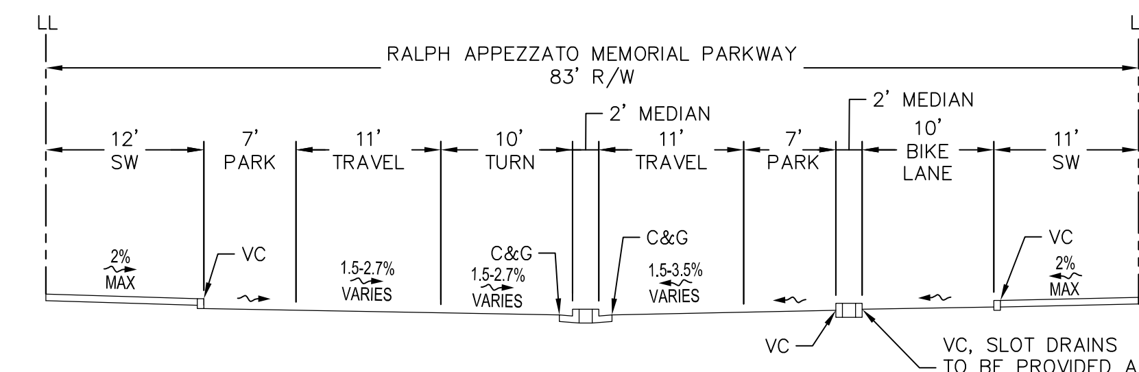
A RALPH APPEZZATO MEMORIAL PARKWAY NTS
