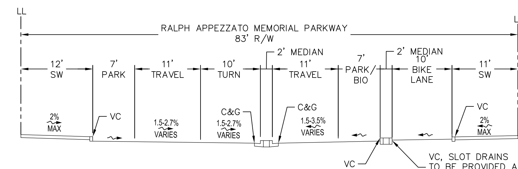
B RALPH APPEZZATO MEMORIAL PARKWAY NTS
