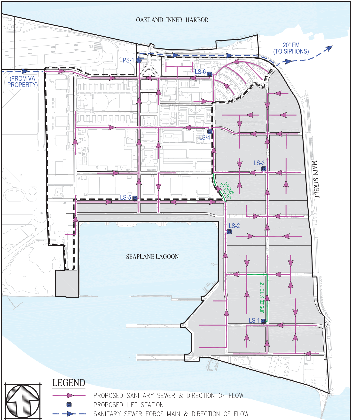
FIGURE 58 PROPOSED ULTIMATE SEWER SYSTEM HIGH DENSITY ALTERNATIVE
