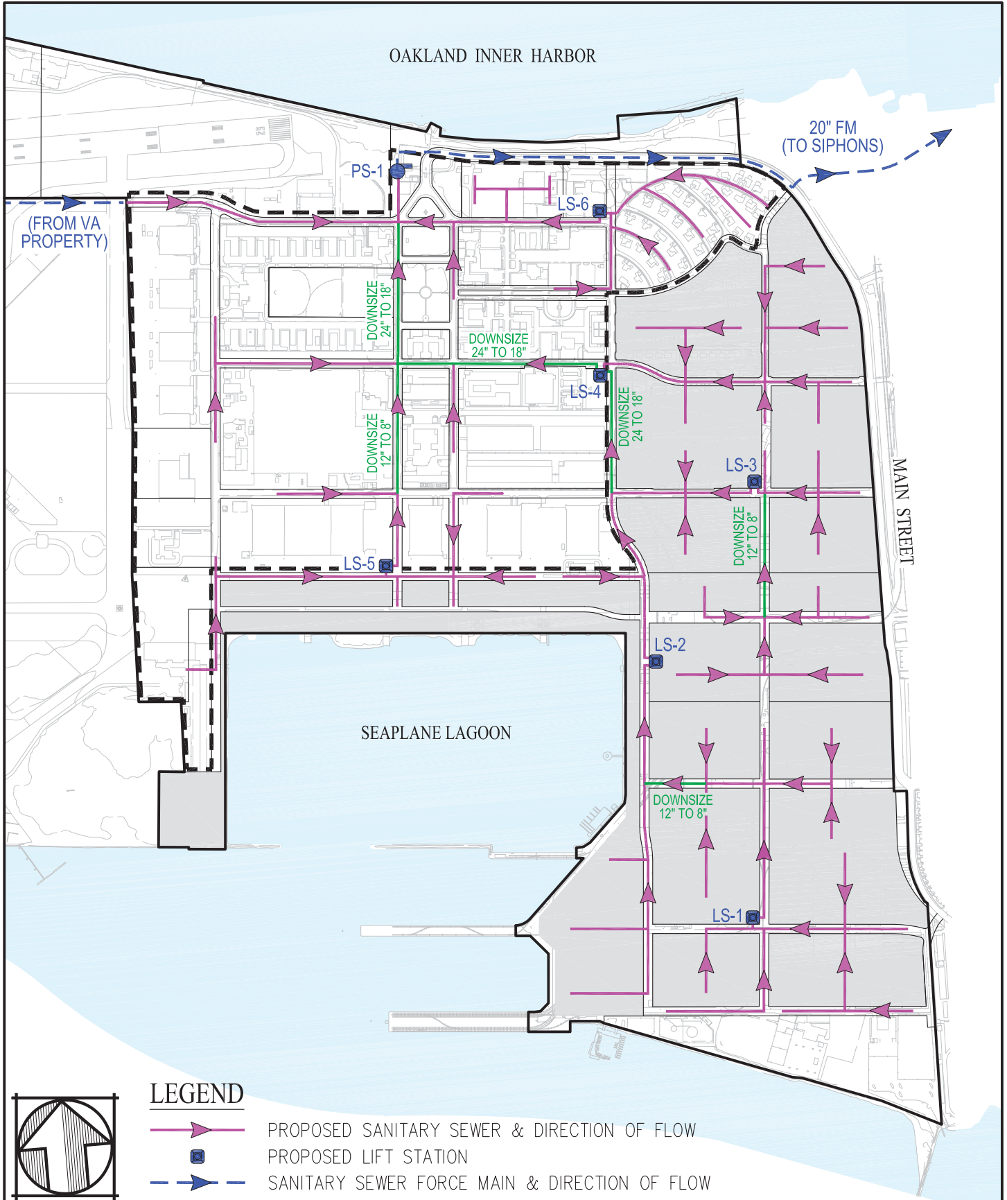
FIGURE 59 PROPOSED ULTIMATE SEWER SYSTEM LOW DENSITY ALTERNATIVE
