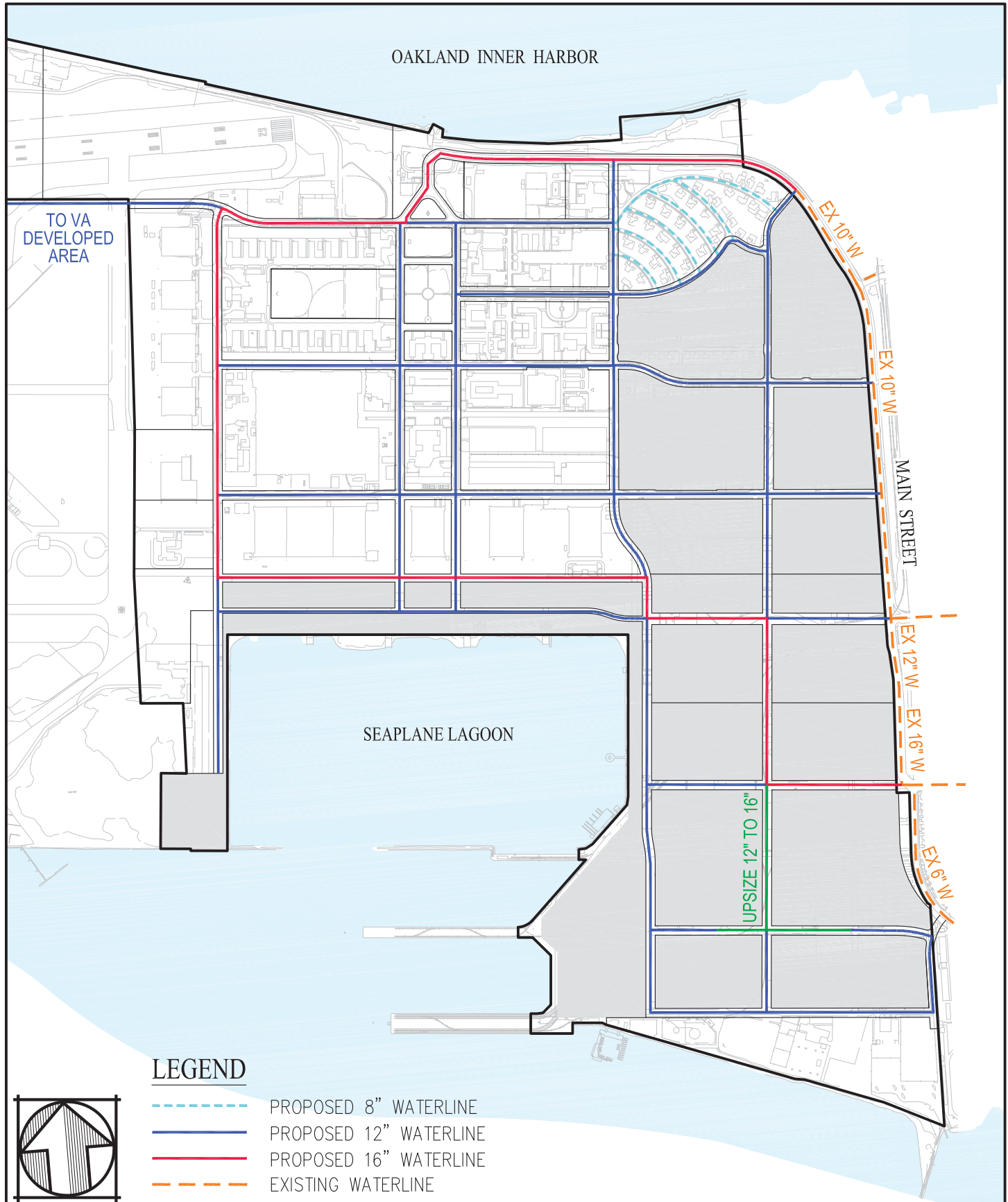
FIGURE 60 PROPOSED ULTIMATE WATER SYSTEM HIGH DENSITY ALTERNATIVE
