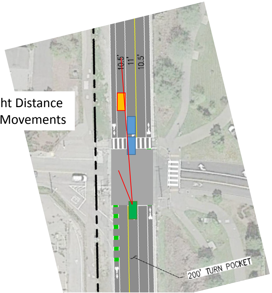
Proposed Configuration w/ Left Turn Pockets
