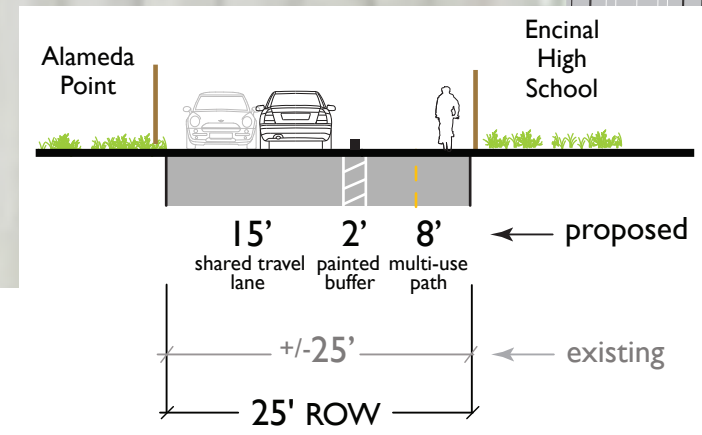
Section B
