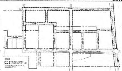
PHASE 3 BACKBONE ROADWAY INFRASTRUCTURE 04/14/2015 3 OF 3
