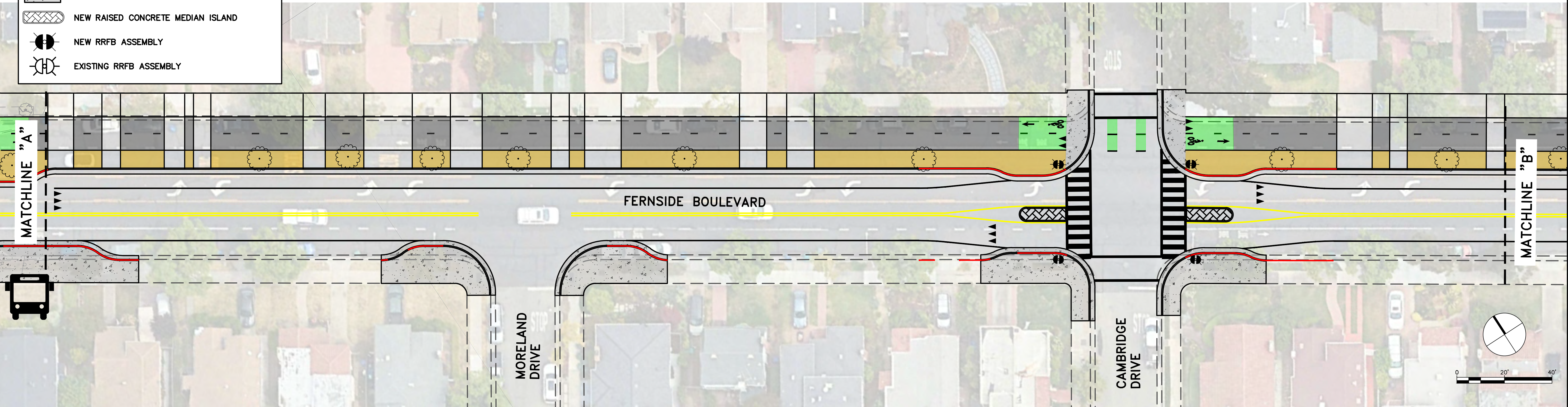
Exhibit 3: Long-Term Concept for Full Corridor (Raised Bikeway Shown)
