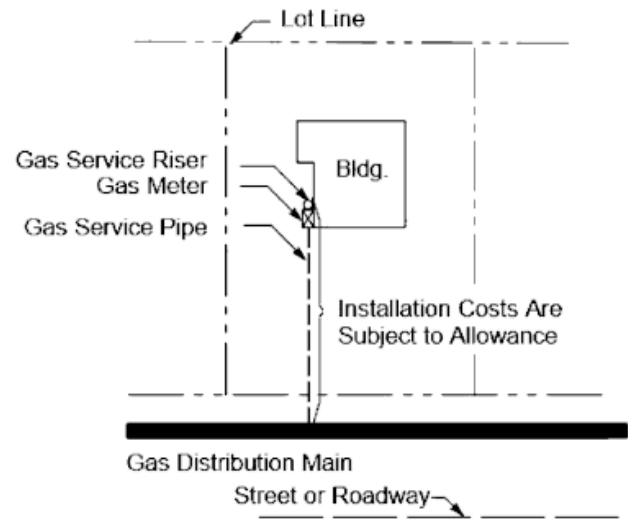
Figure 2-1 Typical Gas Service Installation
