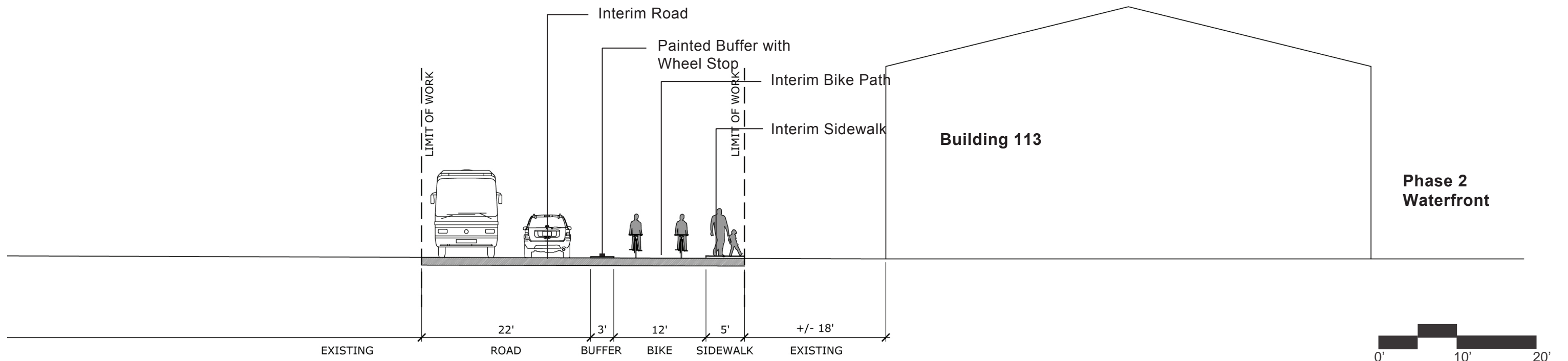
SECTION CC (Interim Connection to Site A)
