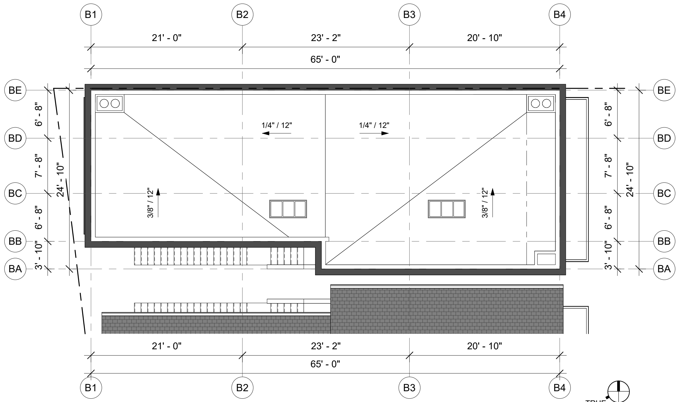
1 BUILDING B - ROOF PLAN 1/8" = 1'-0"
