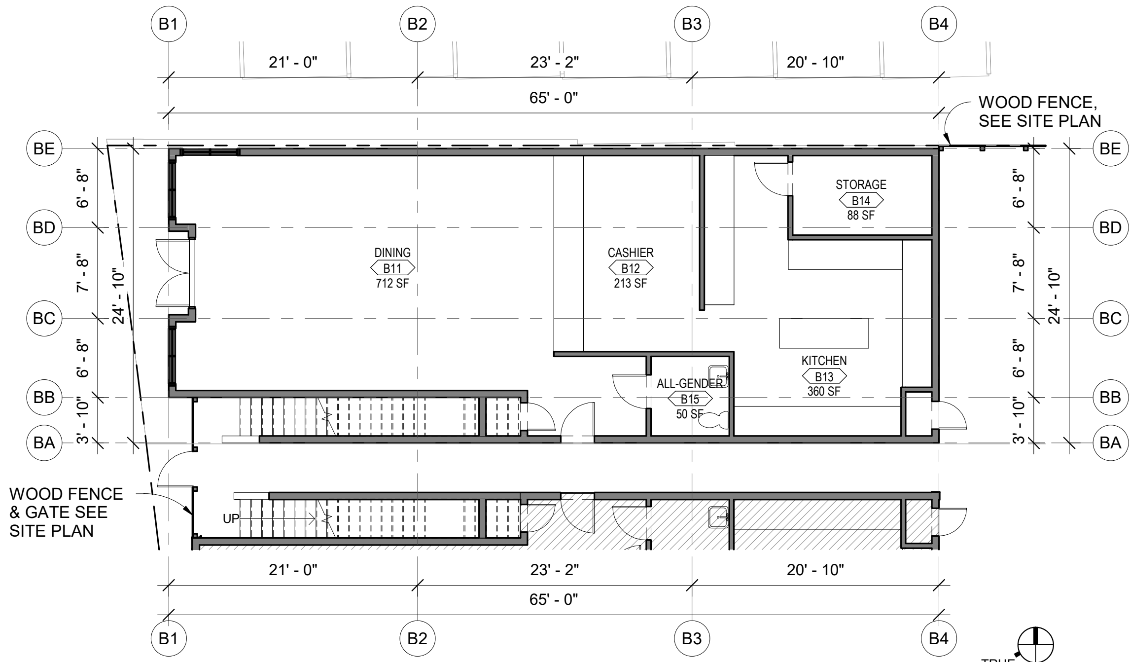
1 BUILDING B - FLOOR PLAN 01 1/8" = 1'-0"
