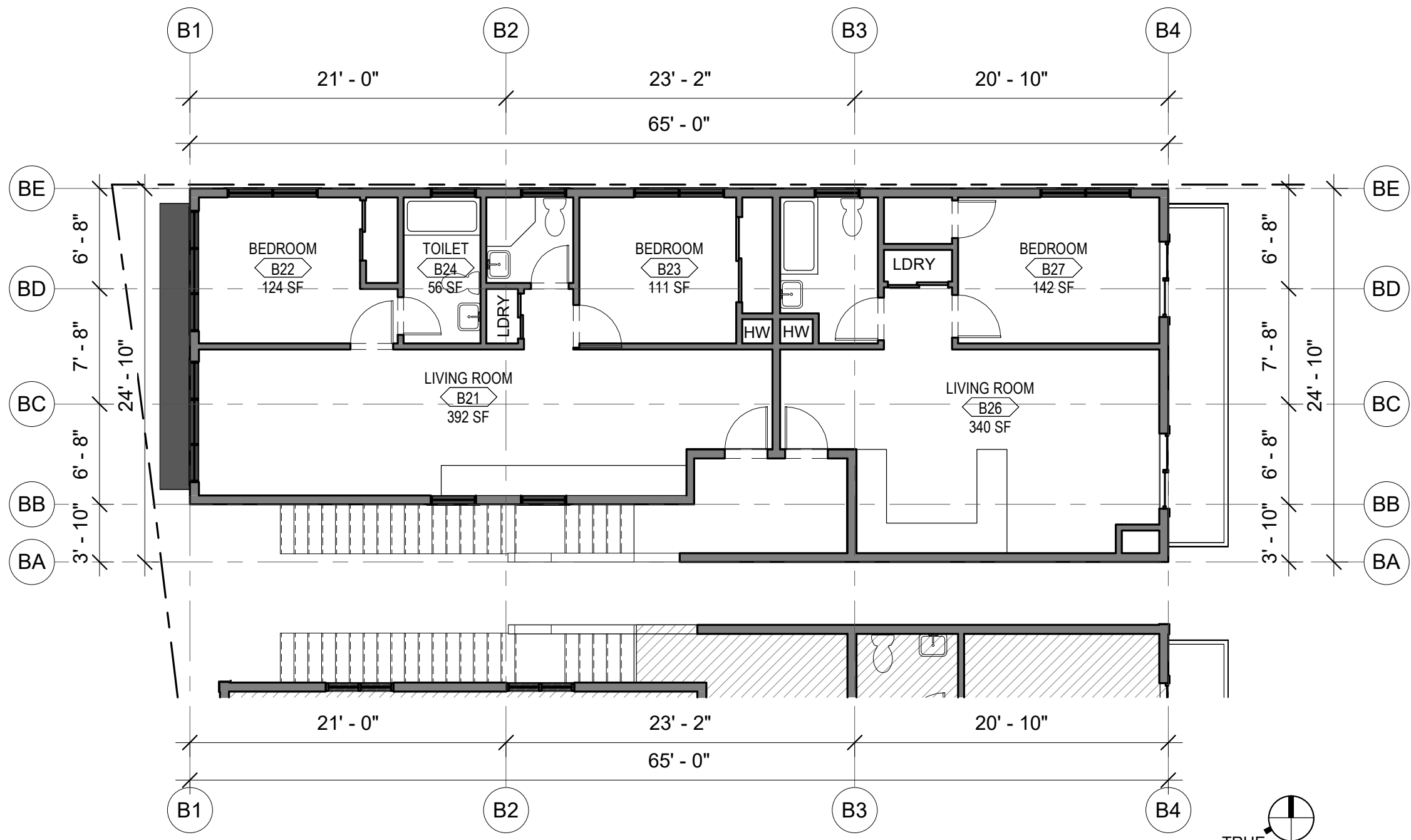
1 BUILDING B - FLOOR PLAN 02 1/8" = 1'-0"
