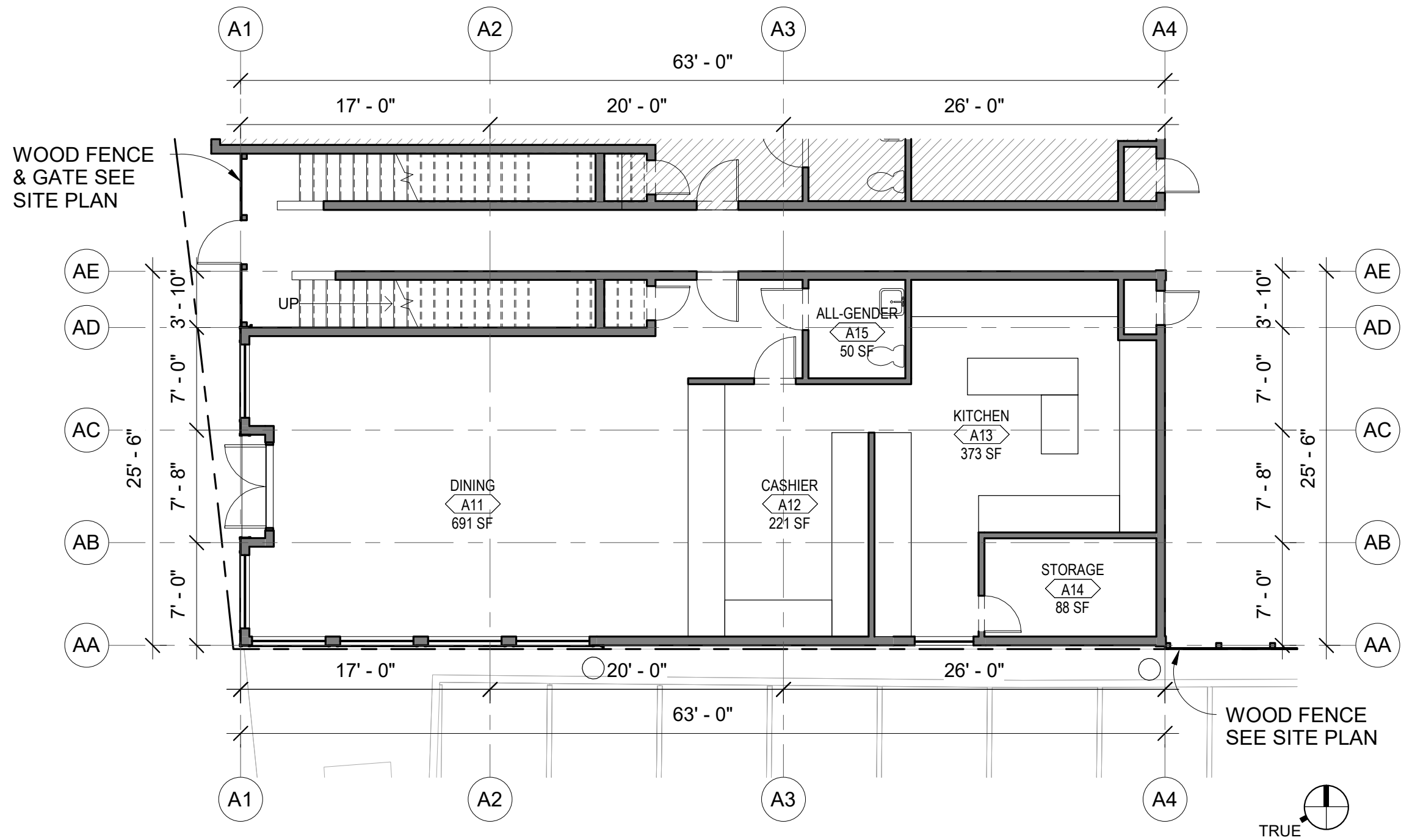
1 BUILDING A - FLOOR PLAN 01 1/8" = 1'-0"
