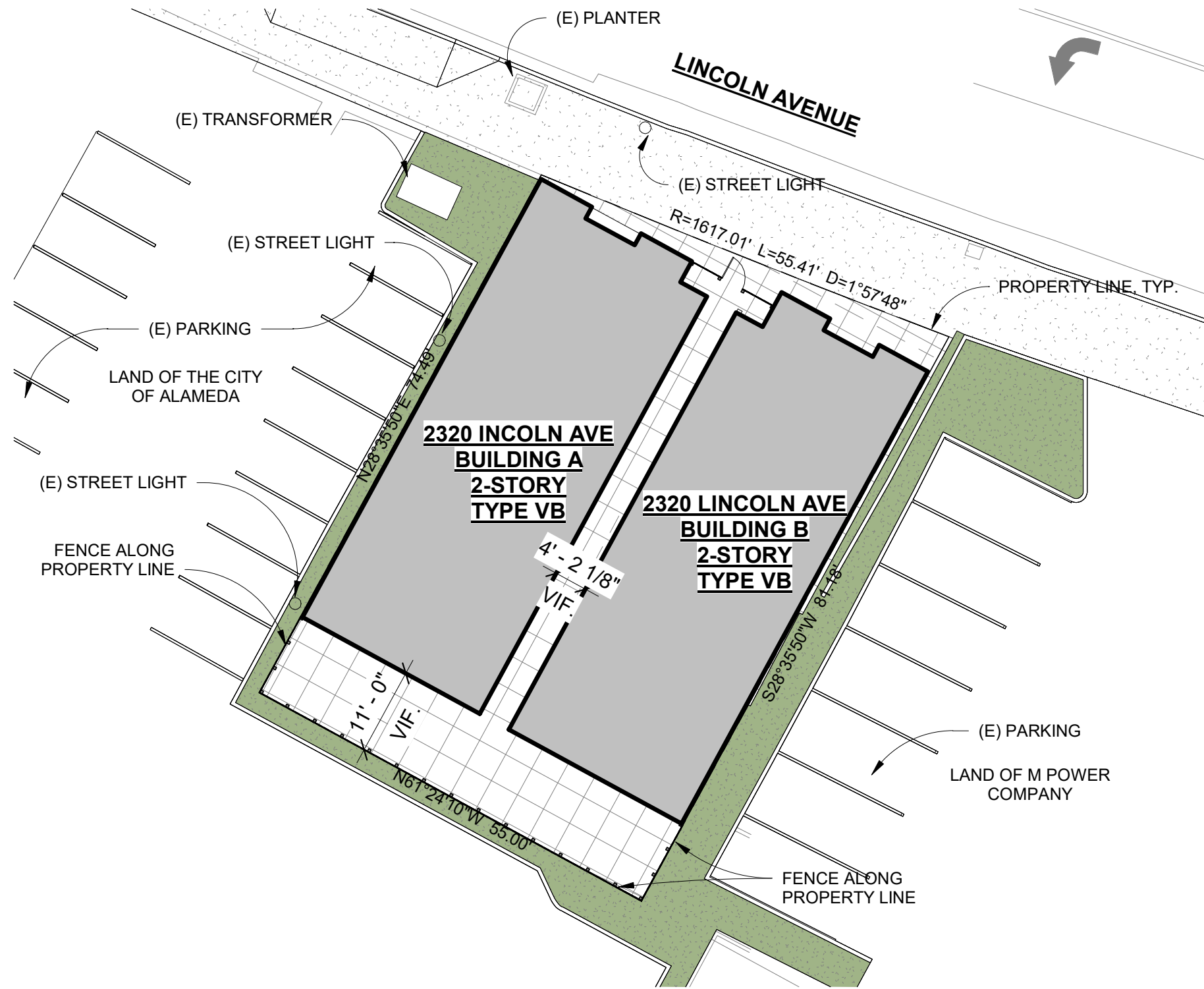
1 01-SITE PLAN 1/16" = 1'-0"
