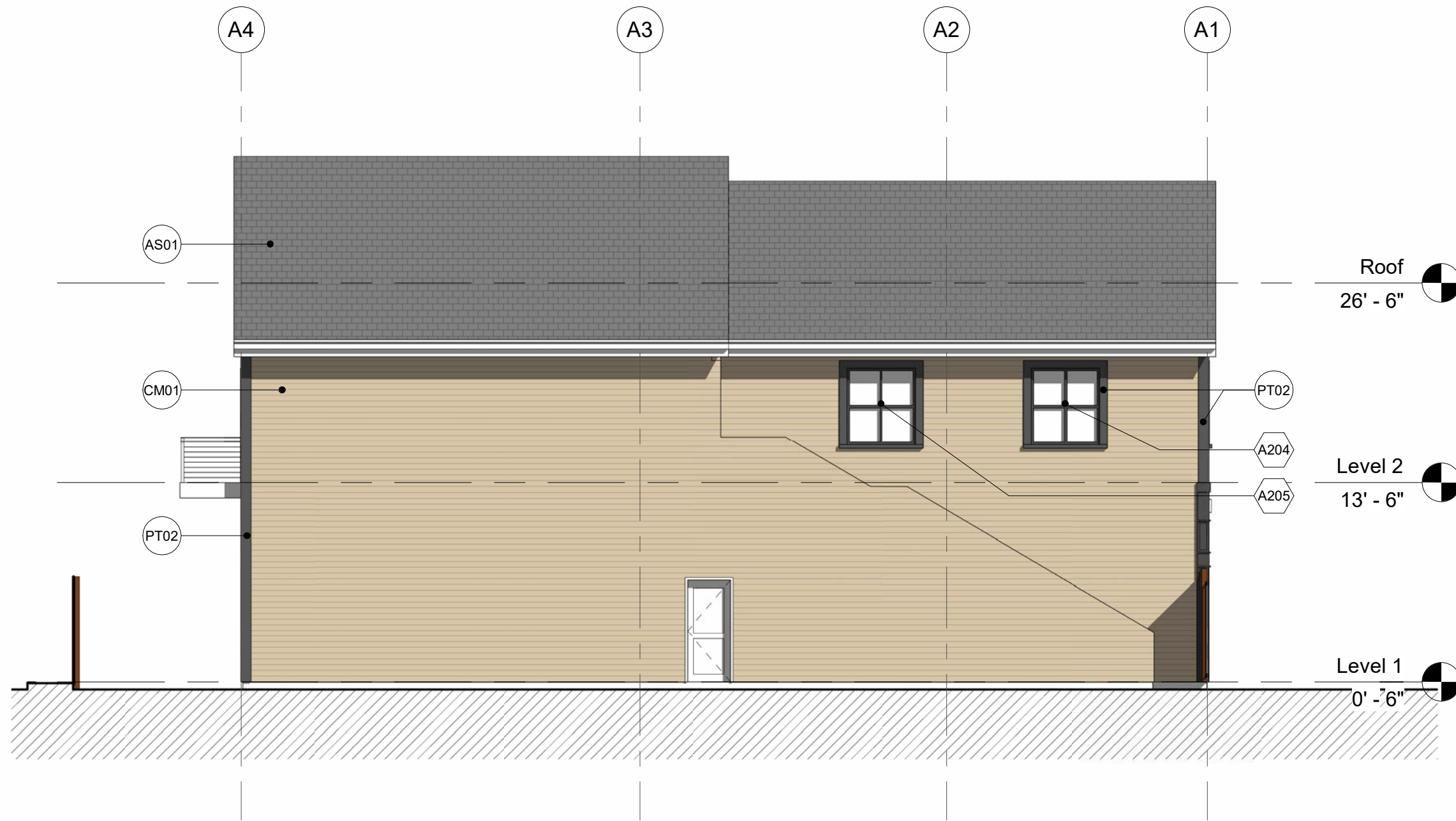
1 BUILDING A - LEFT ELEVATION 1/8" = 1'-0"
