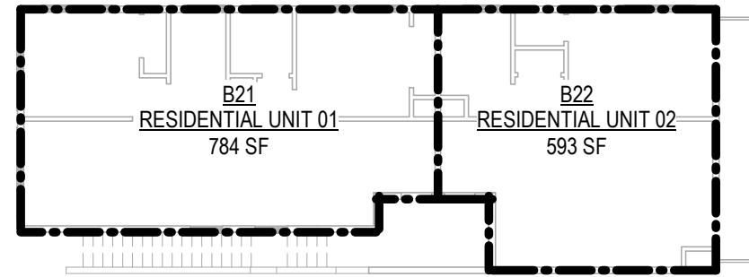
4 BUILDING B - AREA PLAN 02 1/16" = 1'-0"
