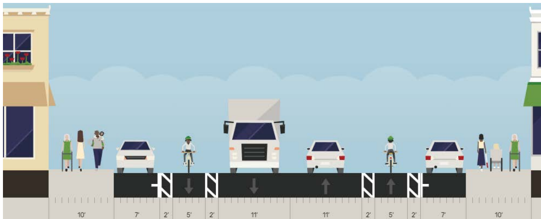
Figure 2: Standard cross section of the draft recommended striping plan in areas where parking is located in front of businesses.
