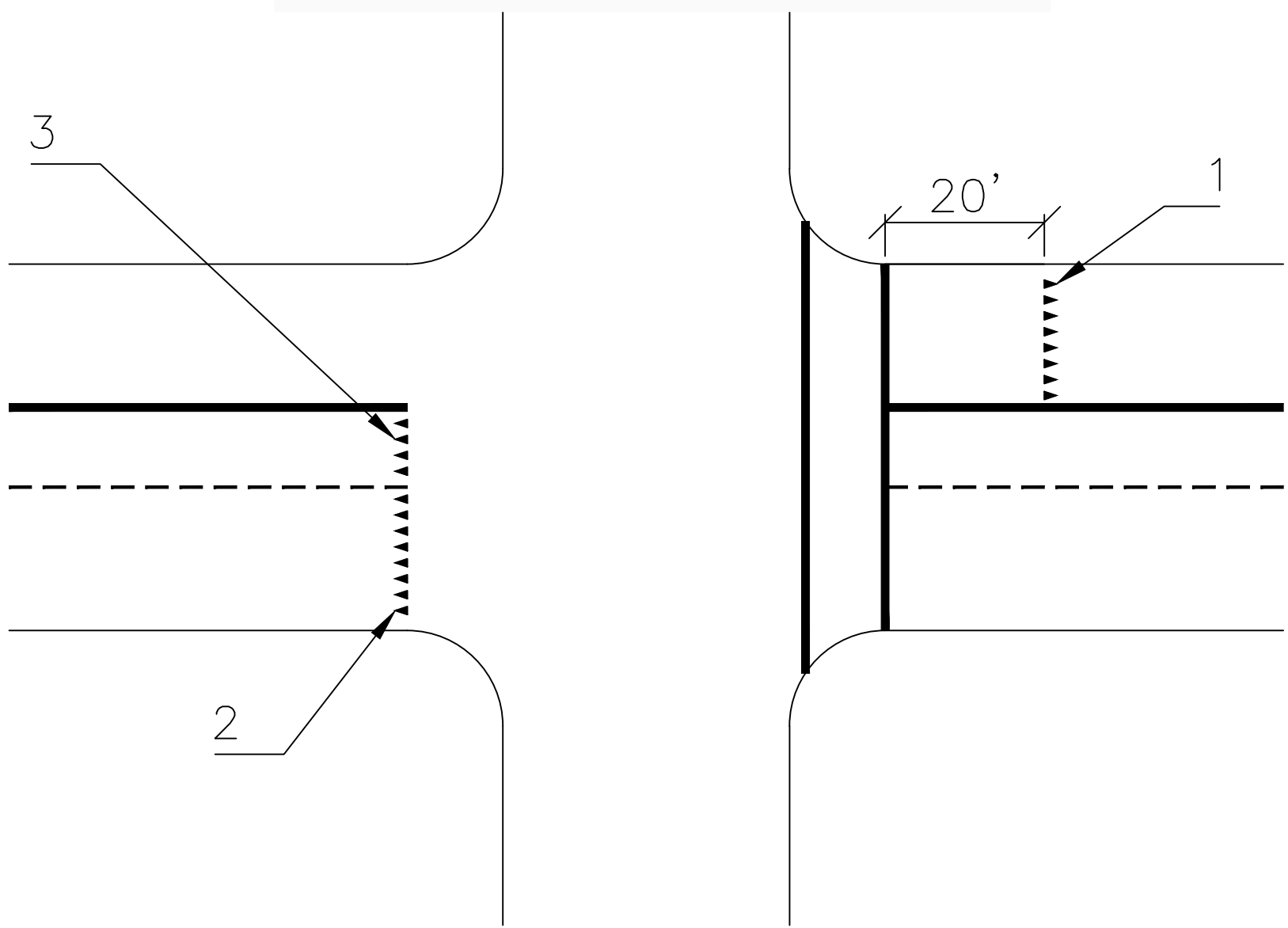
Figure 3. New Yield Marking Details
