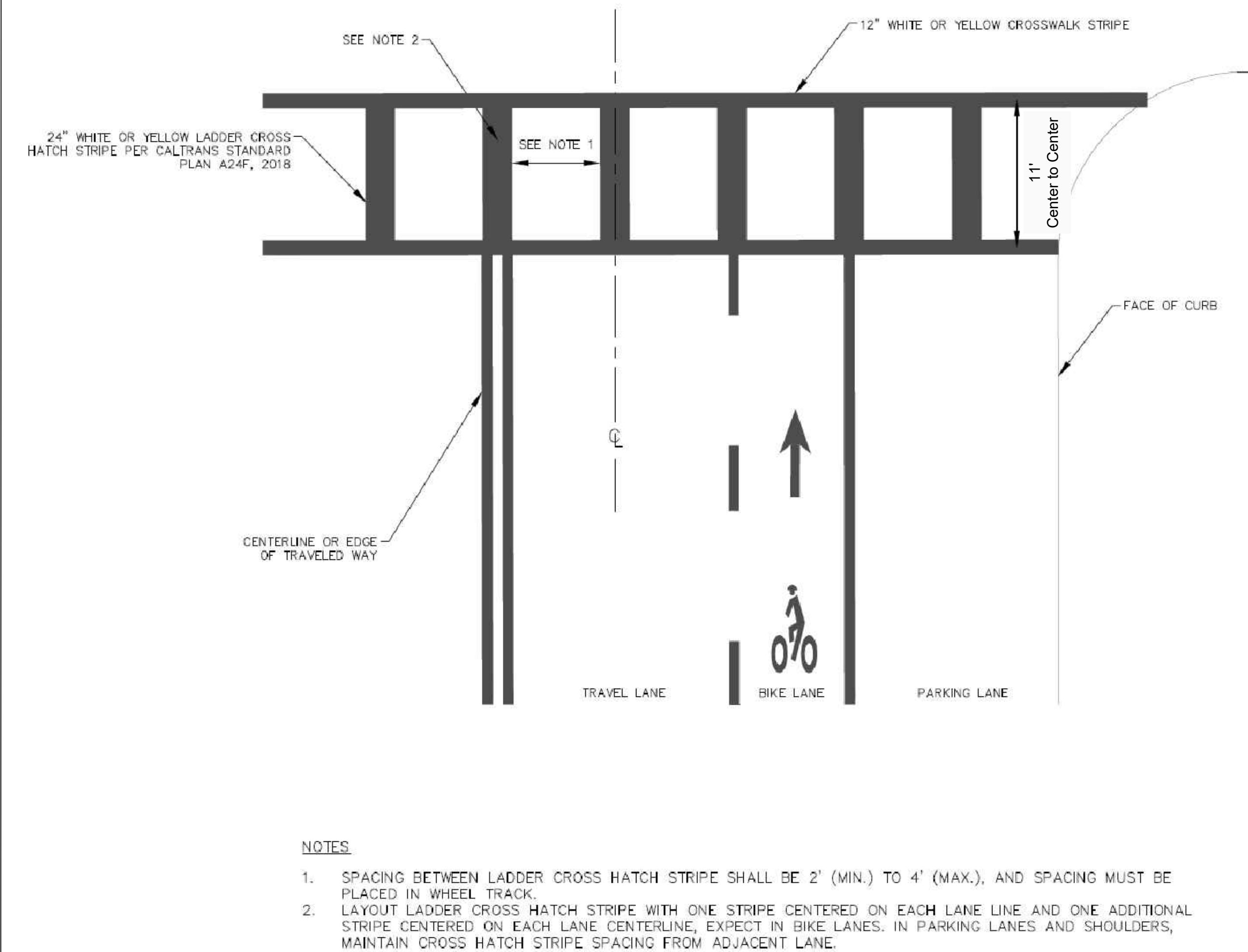
Figure 2. Crosswalk Striping Detail
