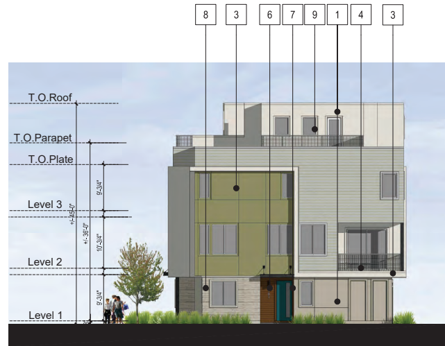
1.RIGHT ELEVATION
