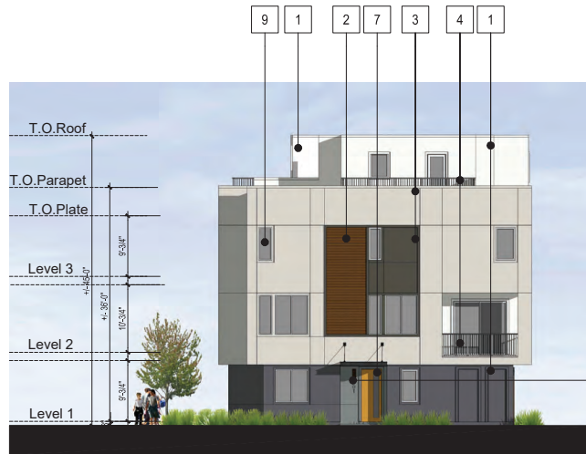
1.RIGHT ELEVATION
