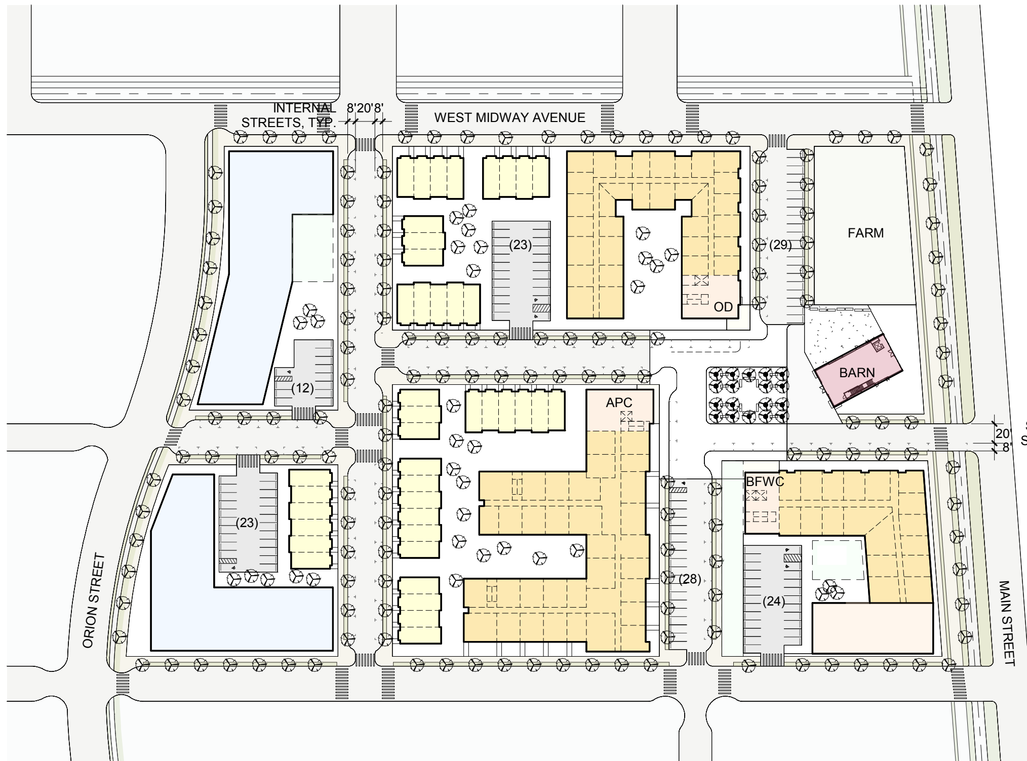
Ground Floor Plan 1" = 100'-0"
