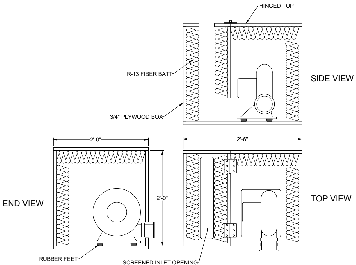
Figure 3 Fan Enclosure
