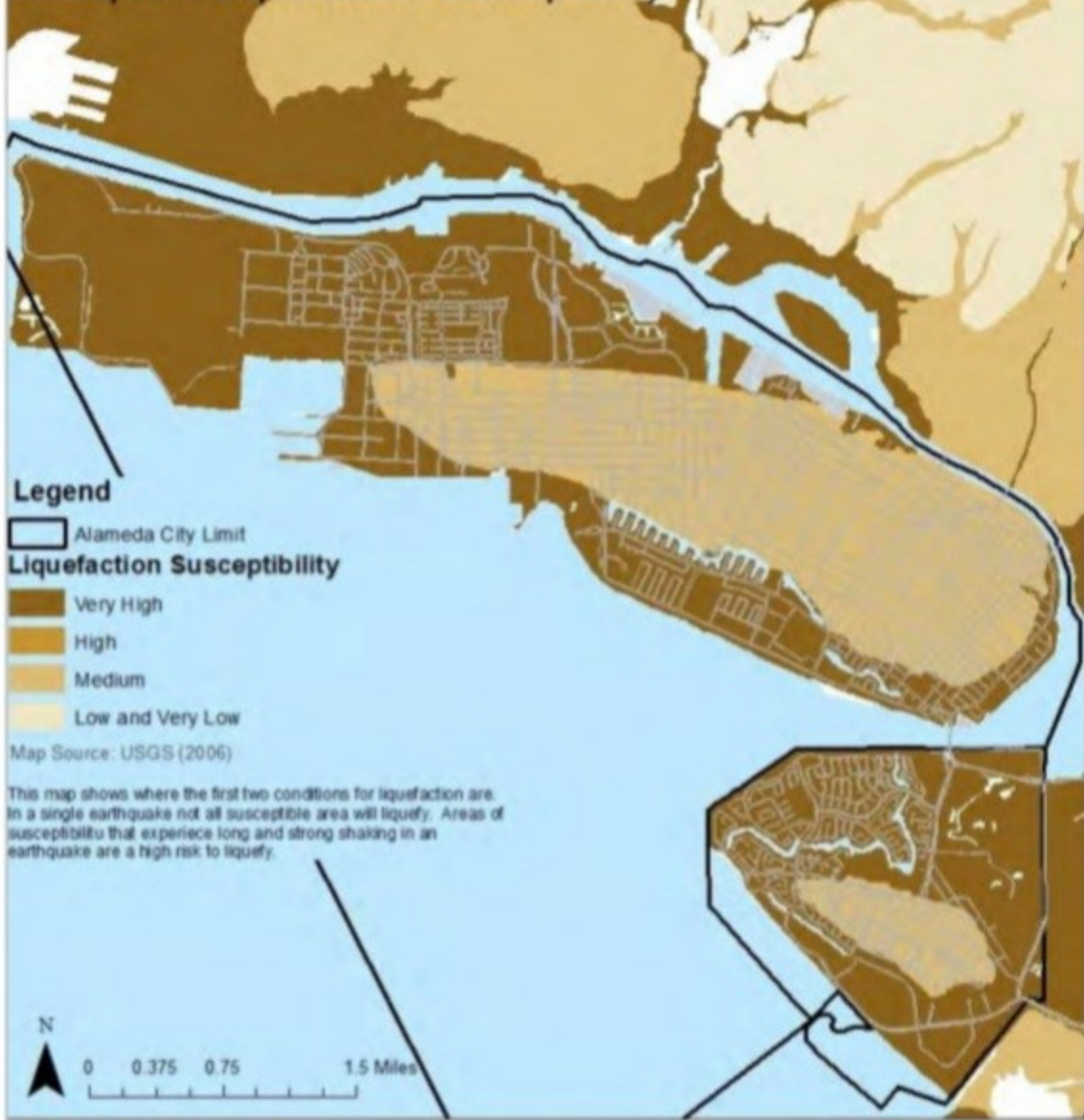
Figure 9. Liquefaction Susceptibility
