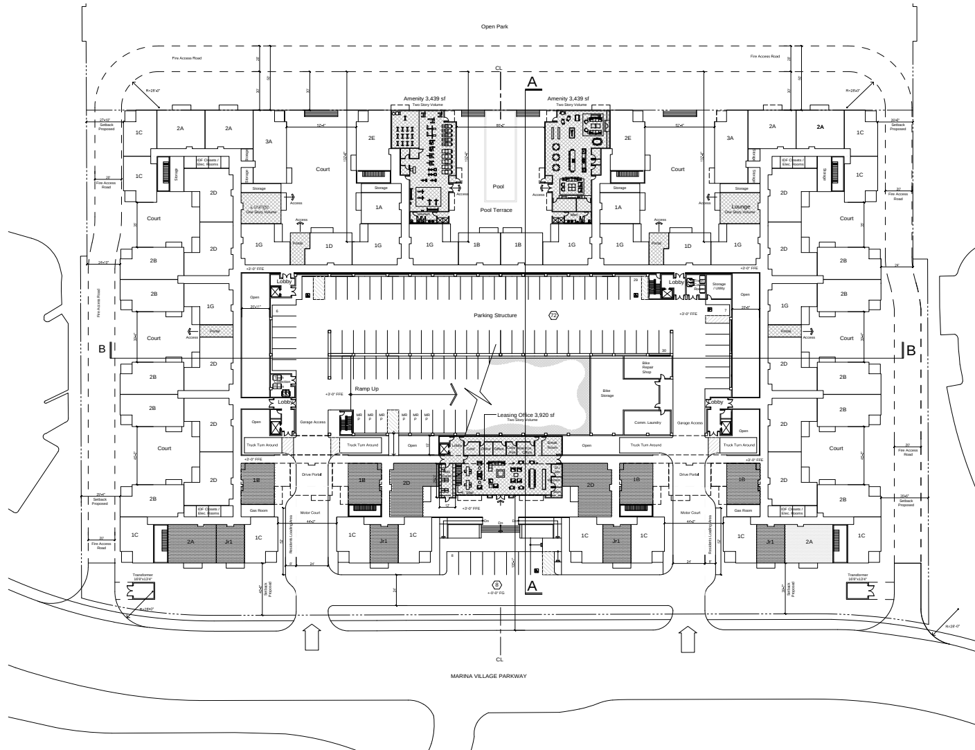
Figure 3-3. Alameda Shipways Site Plan
