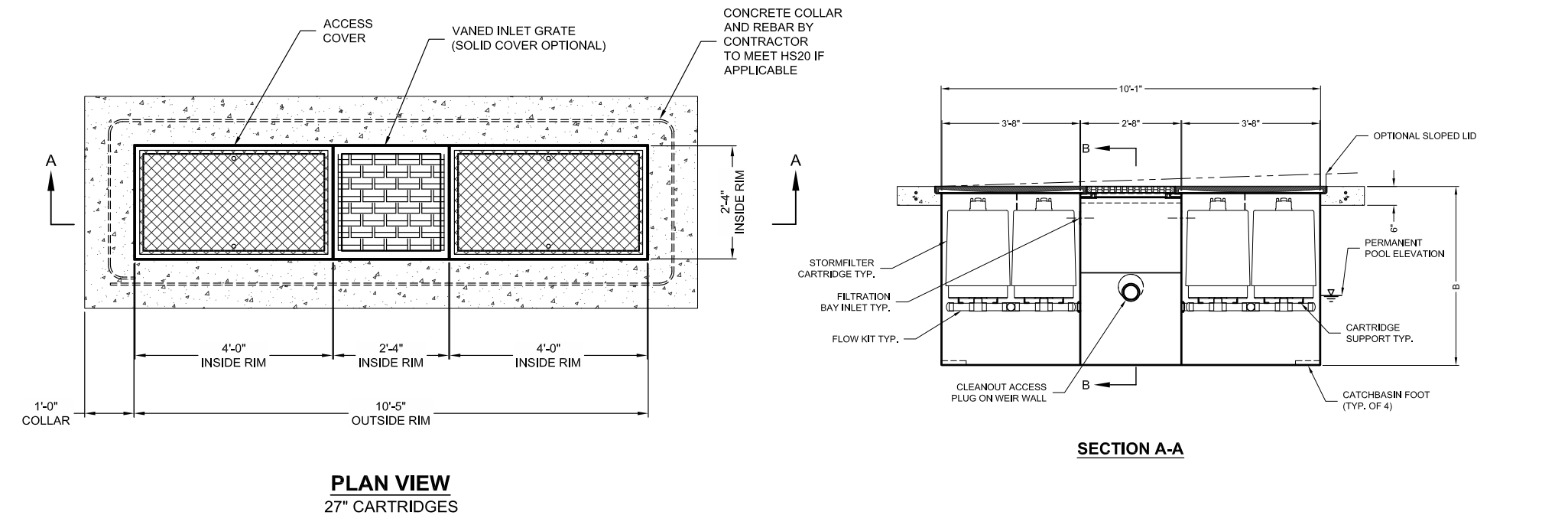
1 MECHANICAL STORMWATER FILTER NTS
