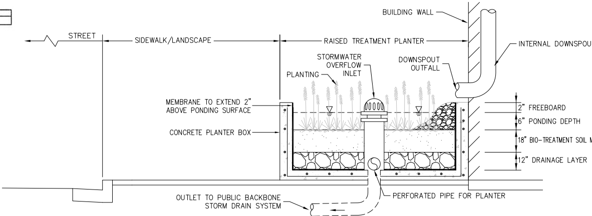
3 FLOW-THROUGH PLANTER NTS
