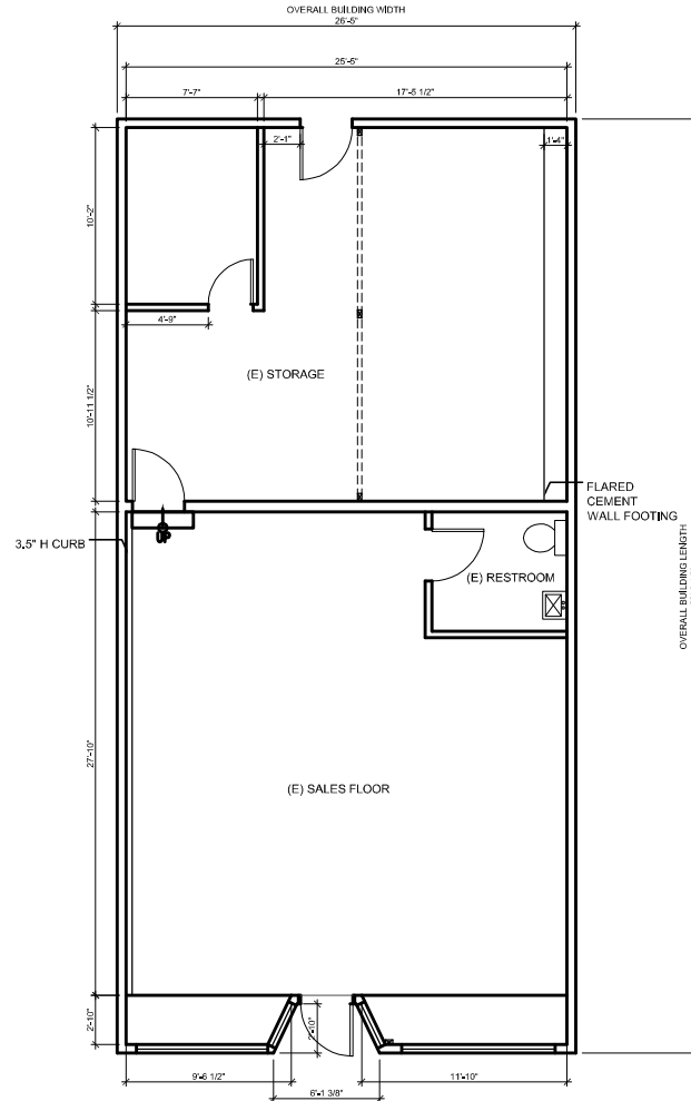
EXISTING FLOORPLAN
