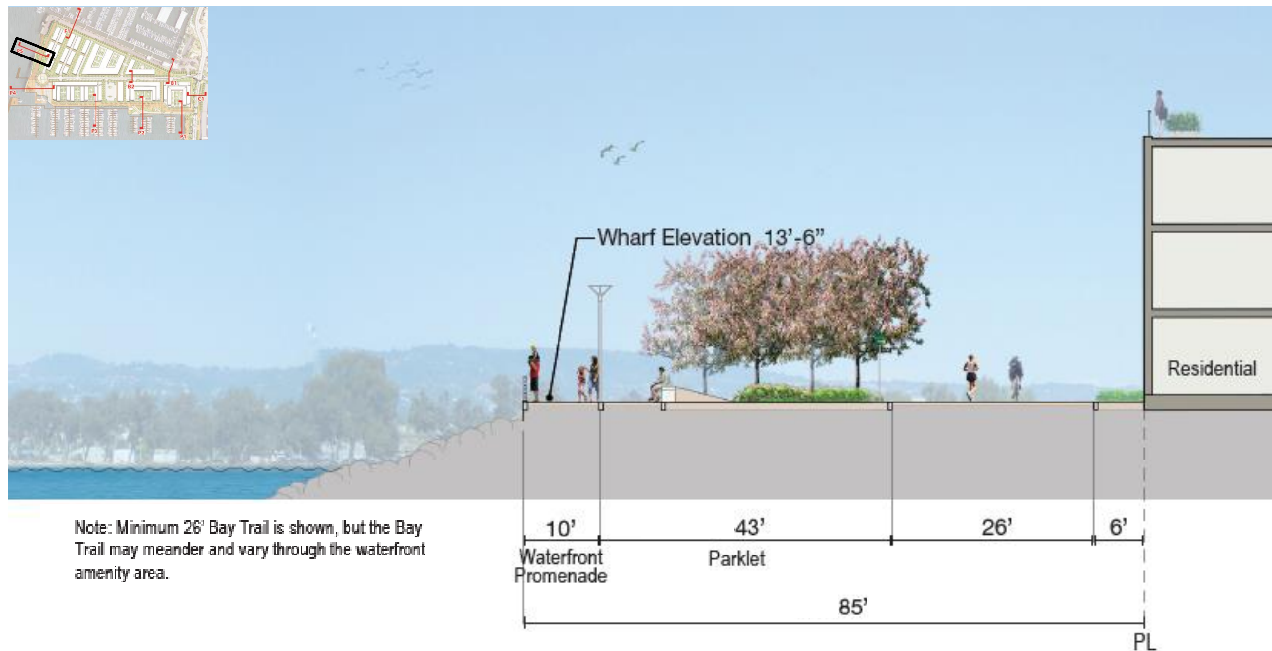
Figure 2.11 Illustrative Cross Section P5: North Shoreline at Estuary District (view looking east)
