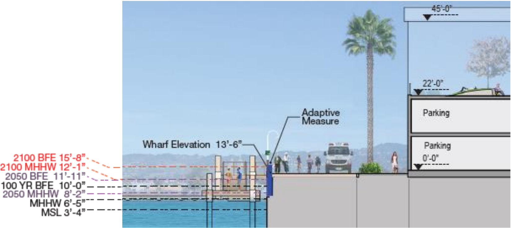
Figure 2.18 Adaptive Measure at wharf edge (Section P3)
