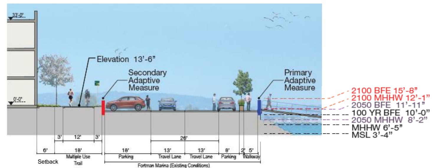
Figure 2.20 Adaptive Measure at Fortman property edge (Section F1)
