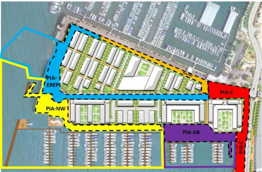
Figure 4.1 Construction Phasing Plan
